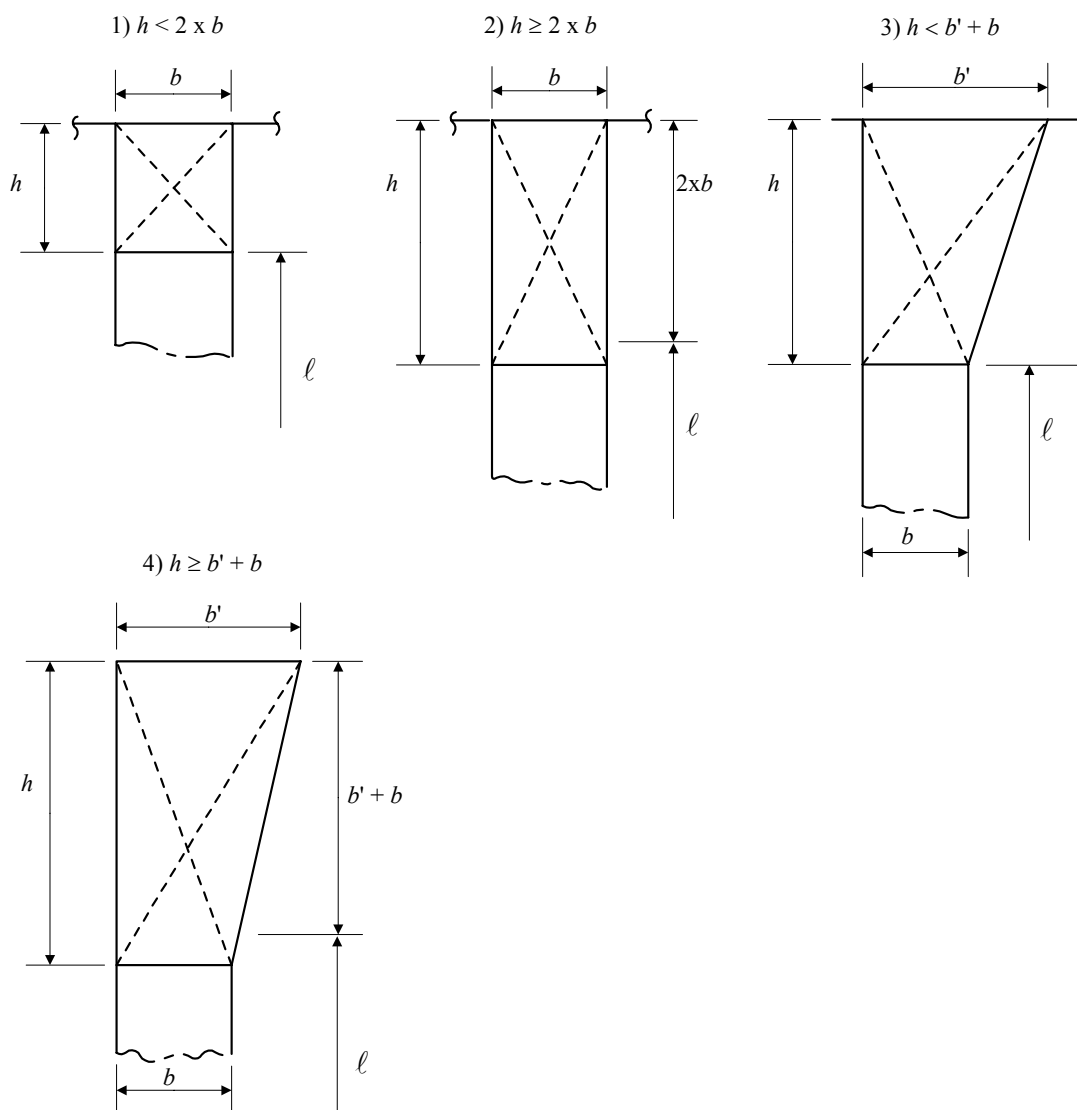
FIGURE 5 Corrugated Bulkhead Upper Stool Credit (1996)
