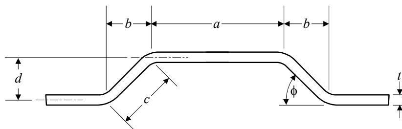
FIGURE 3 Corrugated Bulkhead
