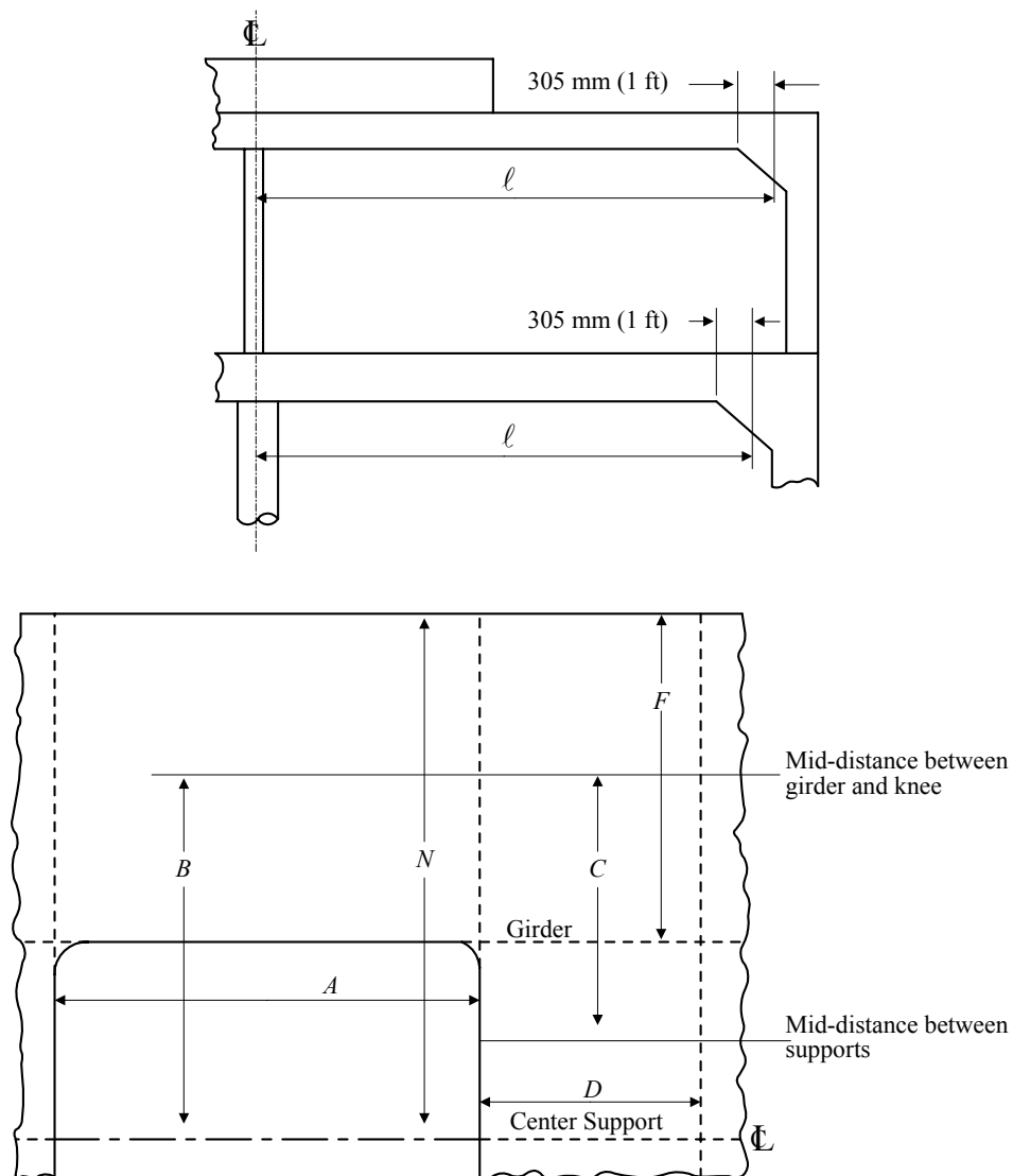
FIGURE 2 Hatch-end Beams
