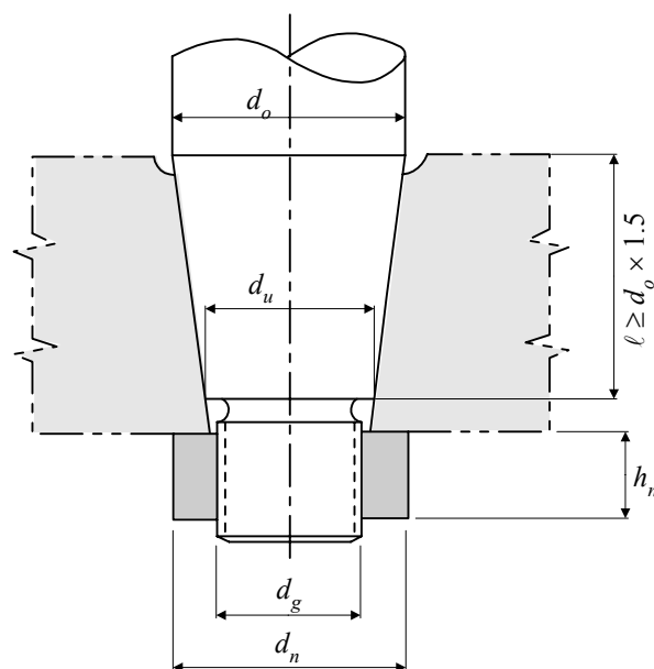
FIGURE 3 Tapered Couplings (1993)
