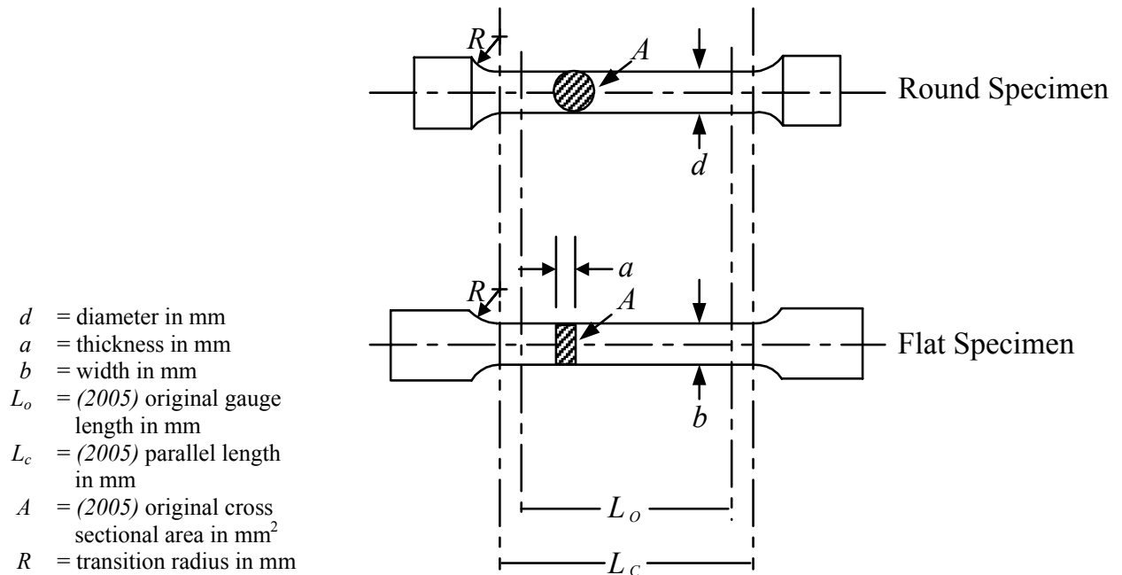
FIGURE 1 Standard Tension Test Specimen (1) (1995)
