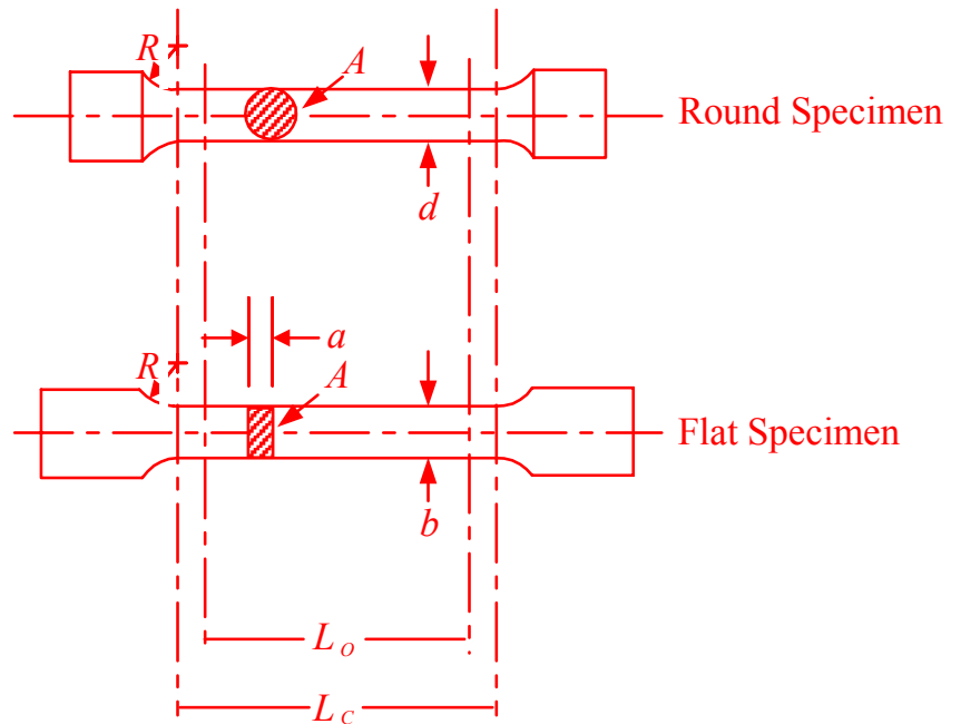
FIGURE 1 Standard Tension Test Specimen (1) (2006)
