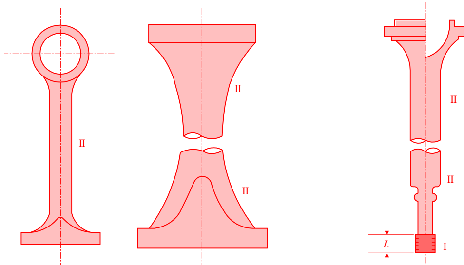
FIGURE 3 Zones for Magnetic Particle/Liquid Penetrant Testing on Machinery Components
