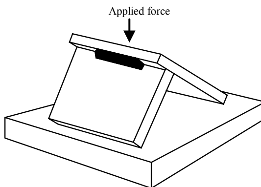
Method of rupturing specimen
