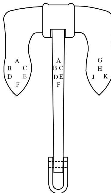
FIGURE 2 Stockless Anchor
