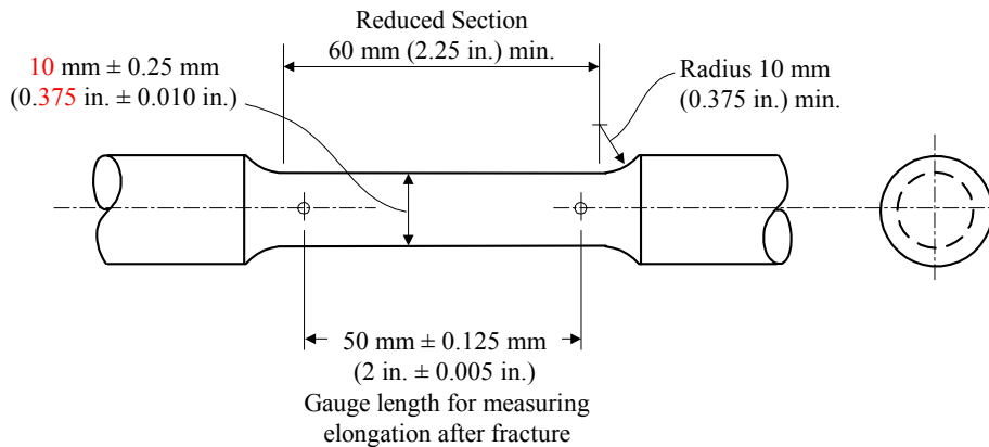
FIGURE 2 Standard Round Tension Test Specimen with 50 mm (2 in.) Gauge Length (2006)
