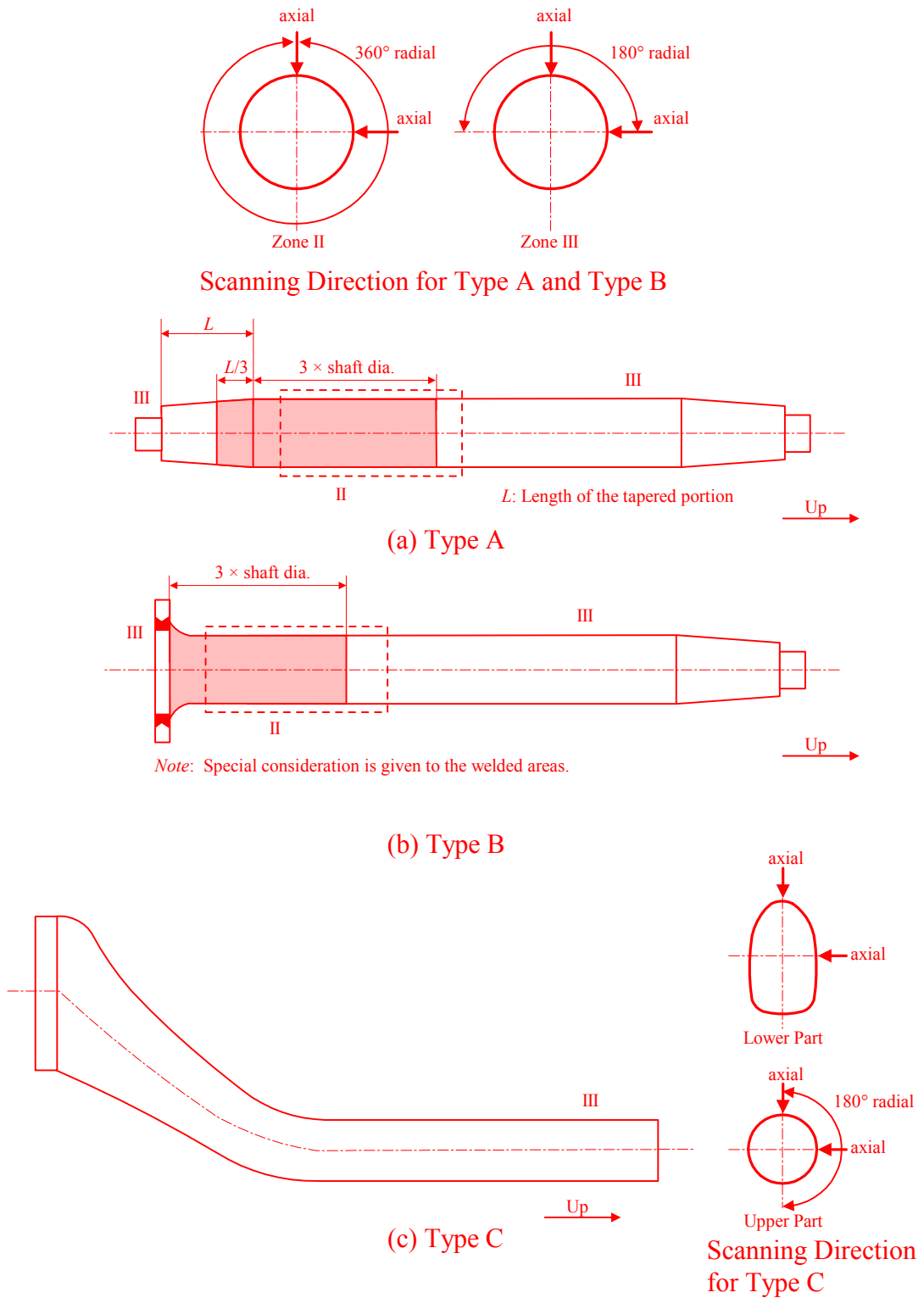
FIGURE 4 Zones for Ultrasonic Testing on Rudder Stocks
