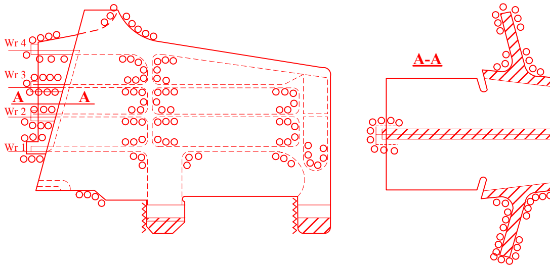
FIGURE 4 Rudder Hangings
