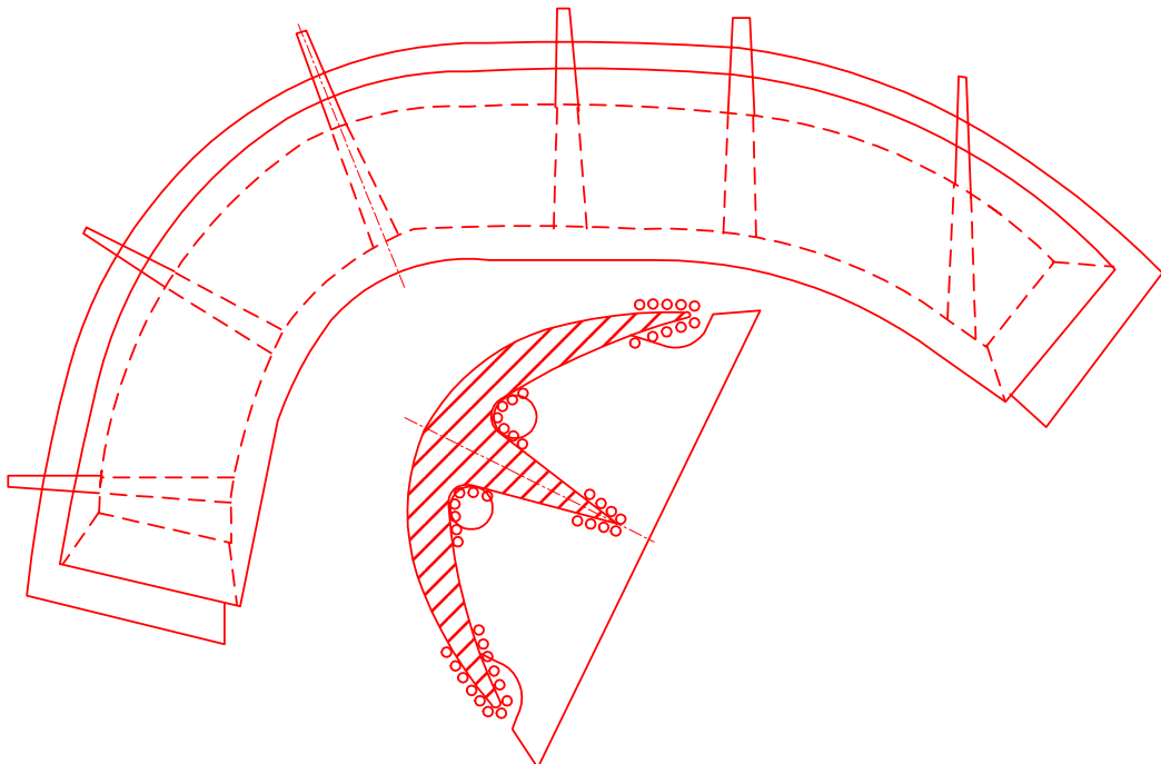
FIGURE 1 Stern Frame
