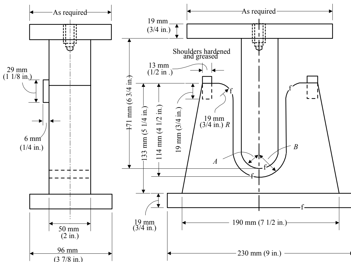
FIGURE 7 Guided Bend Test Jig
