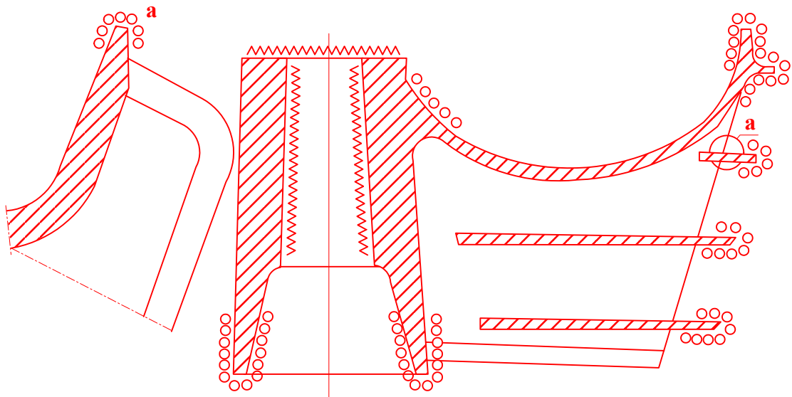
FIGURE 3 Stern Boss
