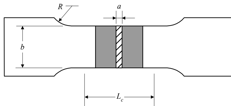
FIGURE 2 Butt Weld Tension Test Specimen (2005)
